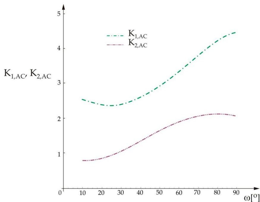
Figure 6. Variation of the real and imaginary parts of the stress intensity factors for the crack that deflects into the AC interface, in terms of angle \omega .
