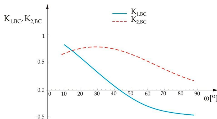
Figure 5. Variation of the real and imaginary parts of the stress intensity factors for the crack that deflects into the BC interface, in terms of angle \omega .
