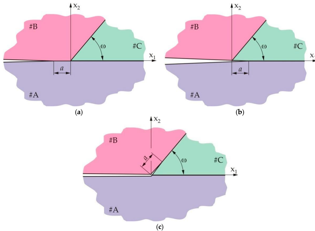
Figure 1. (a) Interface crack approaching a three-material joint; (b) crack propagating along the AC interface; (c) crack deflecting into the BC interface.
