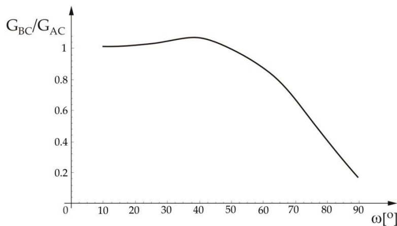
Figure 3. Ratio G_{BC}/G_{AC} in terms of angle \omega .
