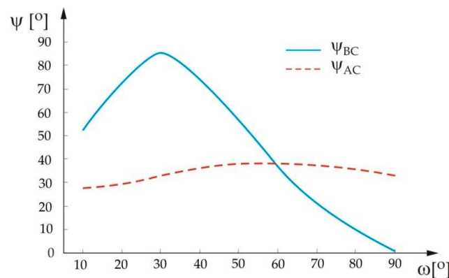
Figure 4. Variation of the mode mixities \psi_{BC} and \psi_{AC} in terms of angle \omega .
