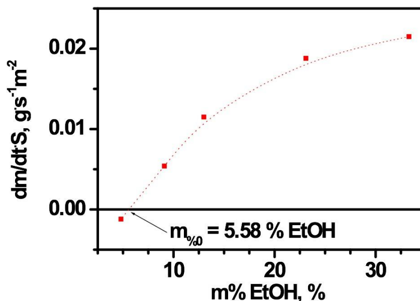
Figure 8. The rate of weight loss \text{dm/dt S, g s}^{-1} \text{m}^{-2} for FA as a function of mass % of ethanol in sample. Temperature T = 22\text{ }^{\circ}\text{C} , relative humidity H = 25\% .
