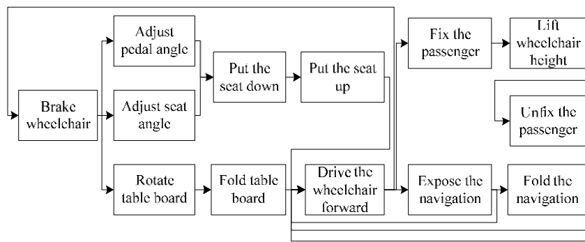
Figure 12. Function chain of the first concept.
