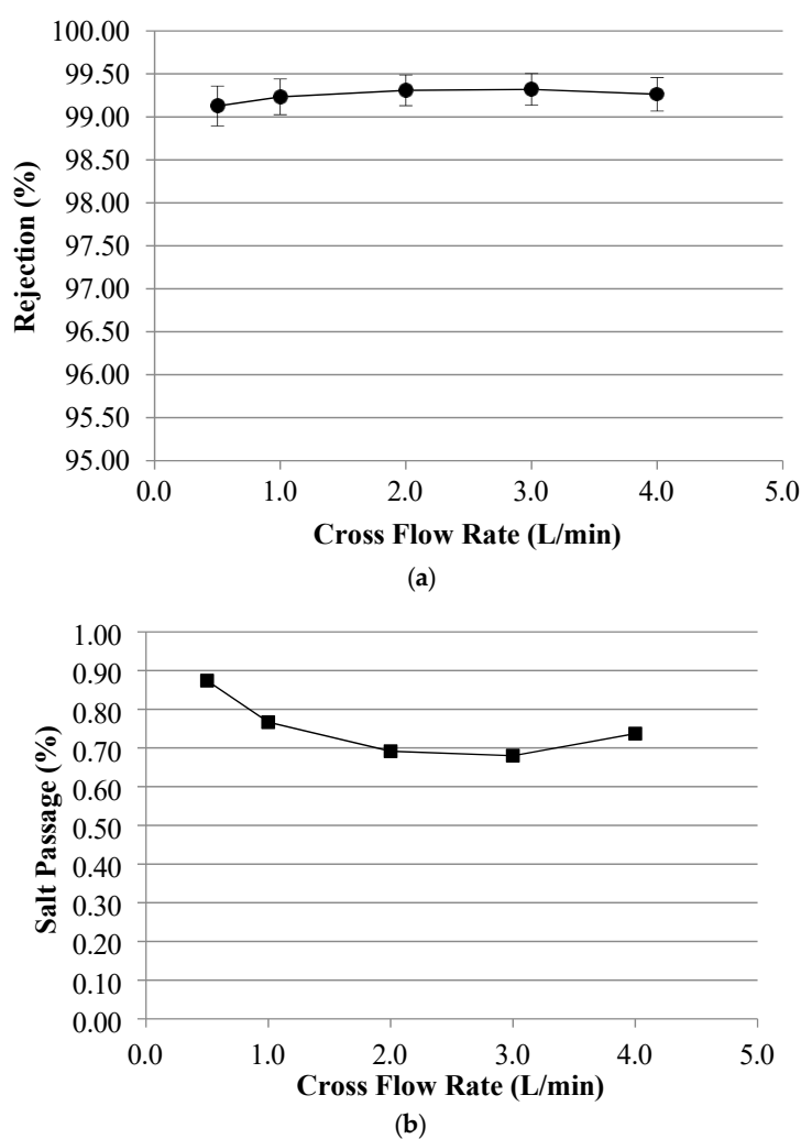
Figure A1. (a) Graph of rejection as a function of the cross flow rate (Operating Conditions: 2000 mg/L MgSO 4 , pH 7, 25 °C, and 10 bar). (b) Graph of salt passage as a function of the cross flow rate (Operating Conditions: 2000 mg/L MgSO 4 , pH 7, 25 °C, and 10 bar).
