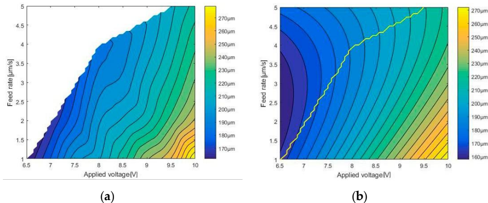
Figure 8. Contour plot: (a) Generated by cubic spline interpolation; (b) plotted using Equation (1).
