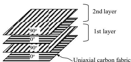
Figure 2. Lay-up arrangement of CFRP laminates.
