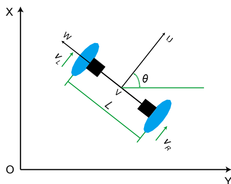
Figure 3. Kinematic model of cleaning robots.
