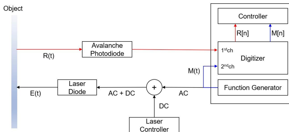
Figure 6. Signal flows of the measurement system.
