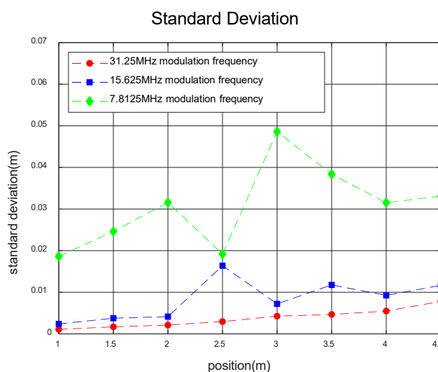
Figure 7. Standard deviation per modulation frequency.
