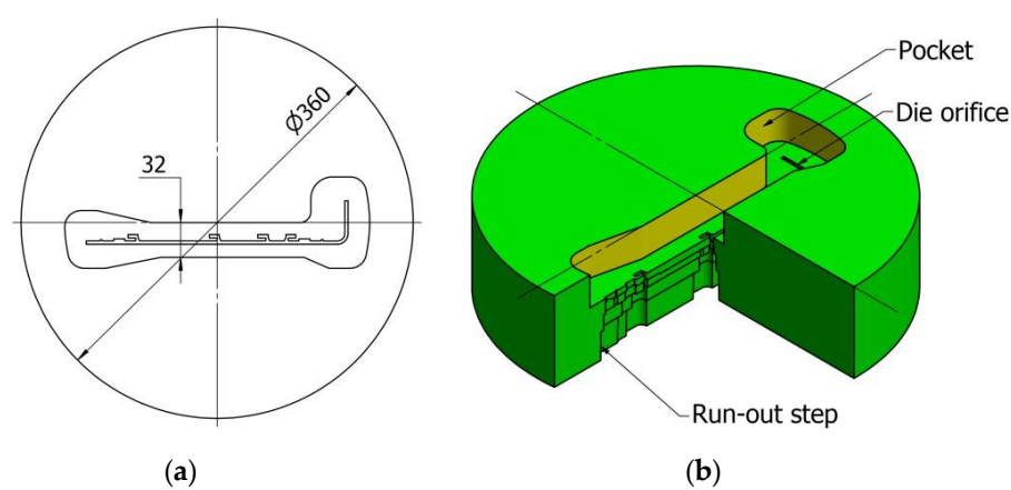
Figure 4. Design for the pocket die: (a) Layout for the entrance; (b) Simplified 3D model (unit: mm).
