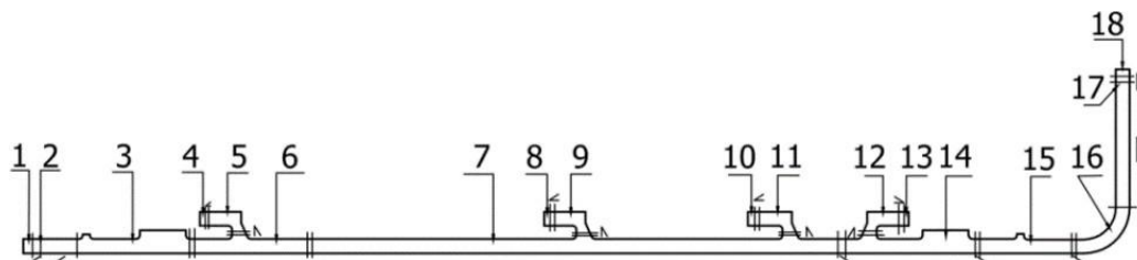
Figure 6. Calculation scheme for bearing regions of the dies.
