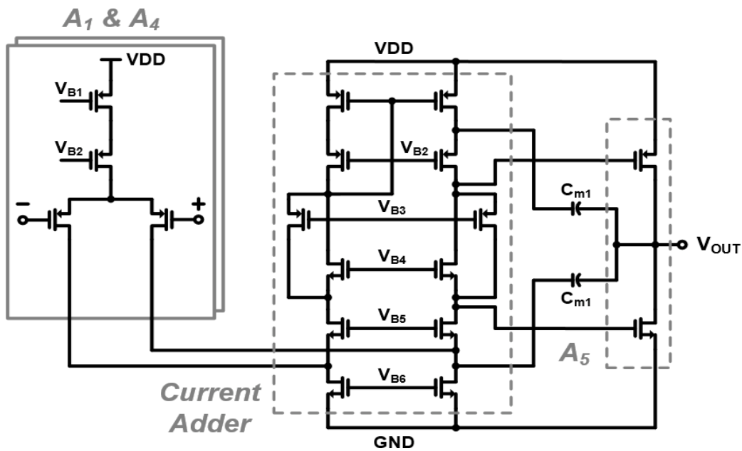
Figure 6. Schematic of the high-frequency path (HFP).
