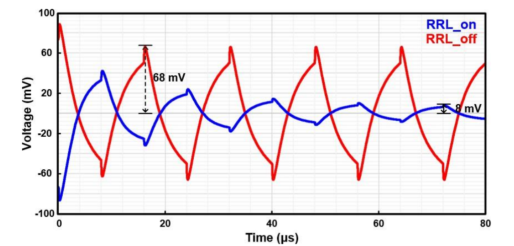
Figure 5. Simulation results of the ripple reduction loop.
