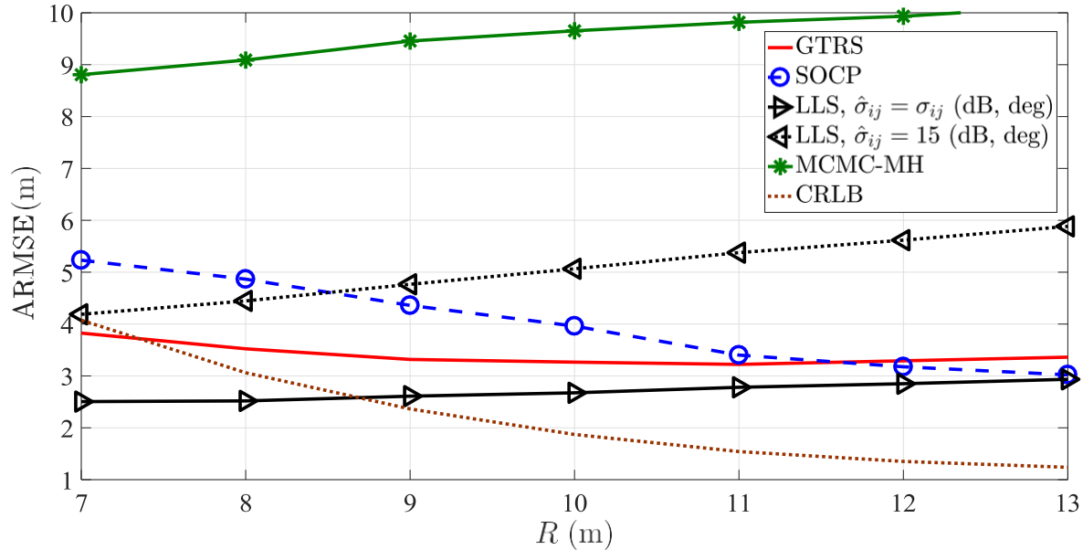
Figure 14. ARMSE (m) versus R (m): N = 15 , M = 50 , M_c = 1000 .
