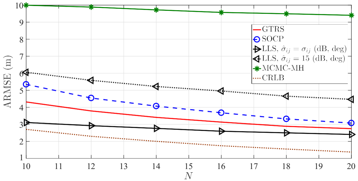
Figure 12. Average root mean square error (ARMSE) (m) versus N : M = 50 , R = 10 m, M_c = 1000 . CRLB = Cramér-Rao lower bound (CRLB).
