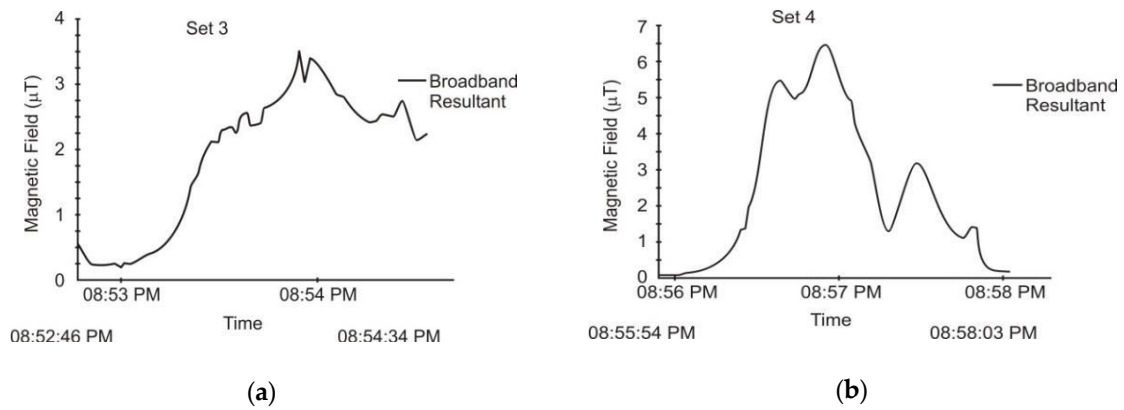
Figure 8. Time variation of the magnetic field induction on an evening peak of power consumption: (a) Measurements on Set Point 3; (b) Measurements on Set Point 4.
