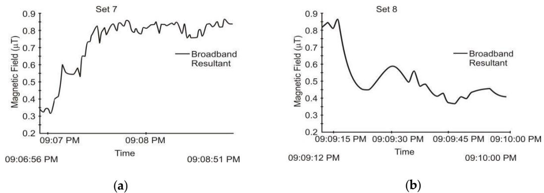
Figure 10. Time variation of the magnetic field induction on an evening peak of power consumption: (a) Measurements on Set Point 7; (b) Measurements on Set Point 8.
