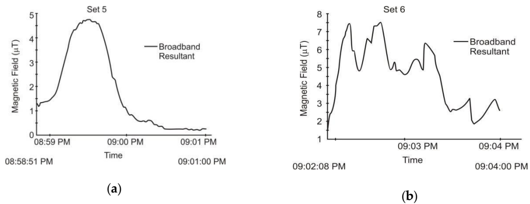
Figure 9. Time variation of the magnetic field induction on an evening peak of power consumption: (a) Measurements on Set Point 5; (b) Measurements on Set Point 6.
