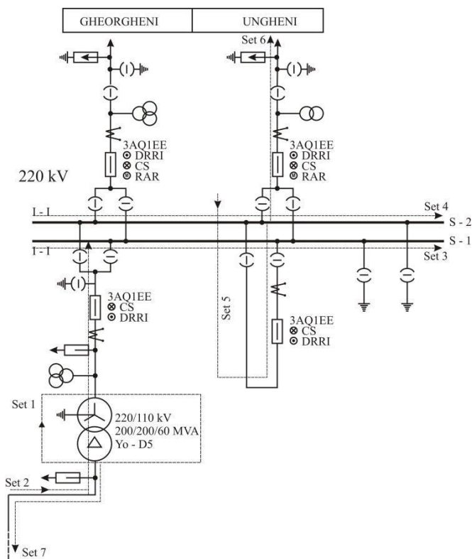
Figure 5. The Measuring Set Points for the Autotransformer area.
