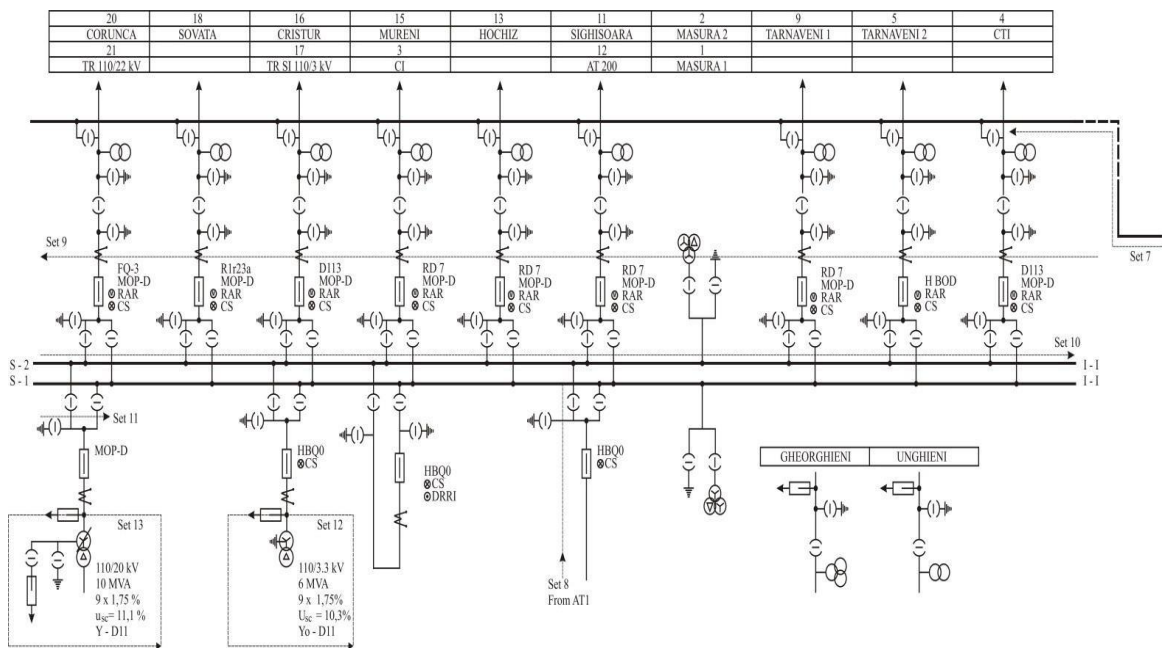
Figure 6. The Measuring Set Points for the Distribution Substation.
