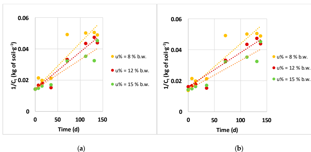
Figure 10. Second-order model for microcosms with C/N = 120: (a) C_0 = 70 \text{ g·kg}^{-1} of soil; (b) C_0 was measured.
