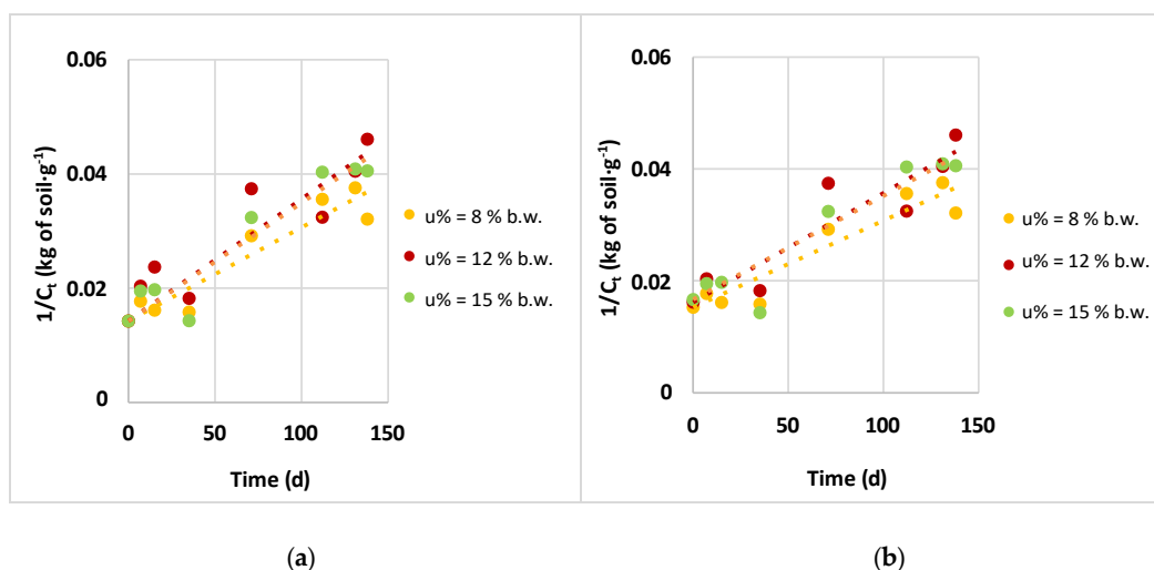
Figure 11. Second-order model for microcosms with C/N = 180: (a) C_0 = 70 \text{ g·kg}^{-1} of soil; (b) C_0 was measured.
