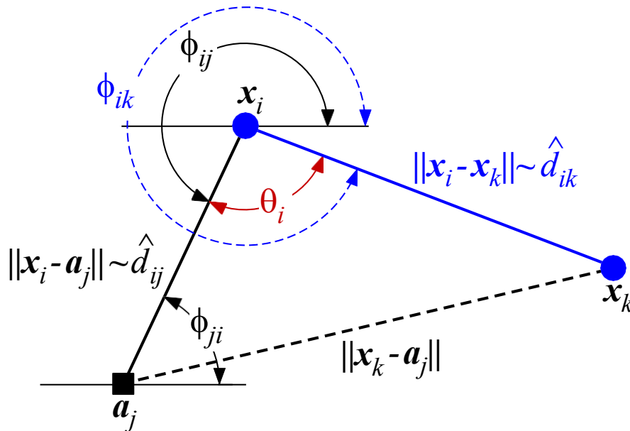
Figure 10. Illustration of the geometric approach in [68] for a 2-hop case.
