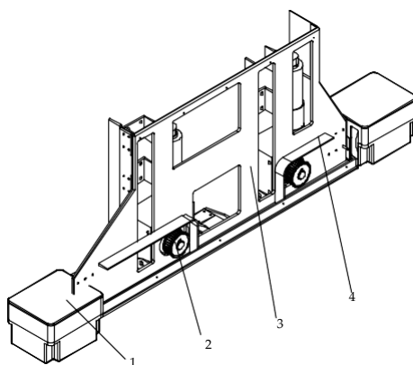
Figure 4. The first design drawing of the right walking mechanism; 1—case cover of the walking wheel, 2—synchronous belt pulley, 3—seat support plate, 4—belt guard.
