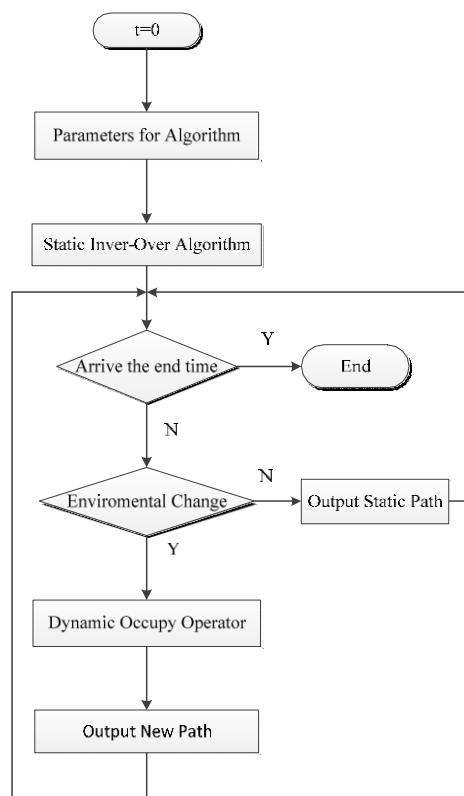
Figure 4. Flowchart of dynamic Inver-Over evolutionary algorithm.
