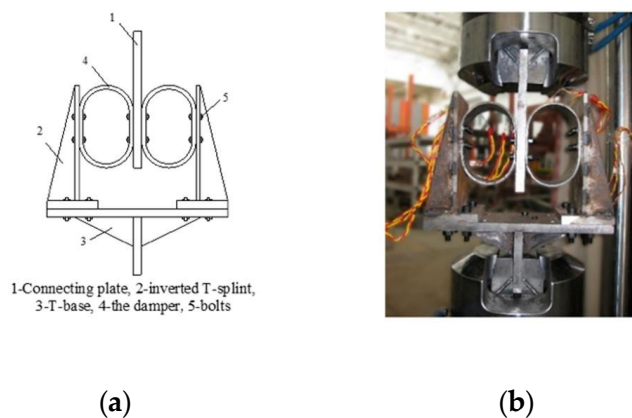
Figure 4. Schematic diagram of the fixture (a) and photograph (b) of the testing device.
