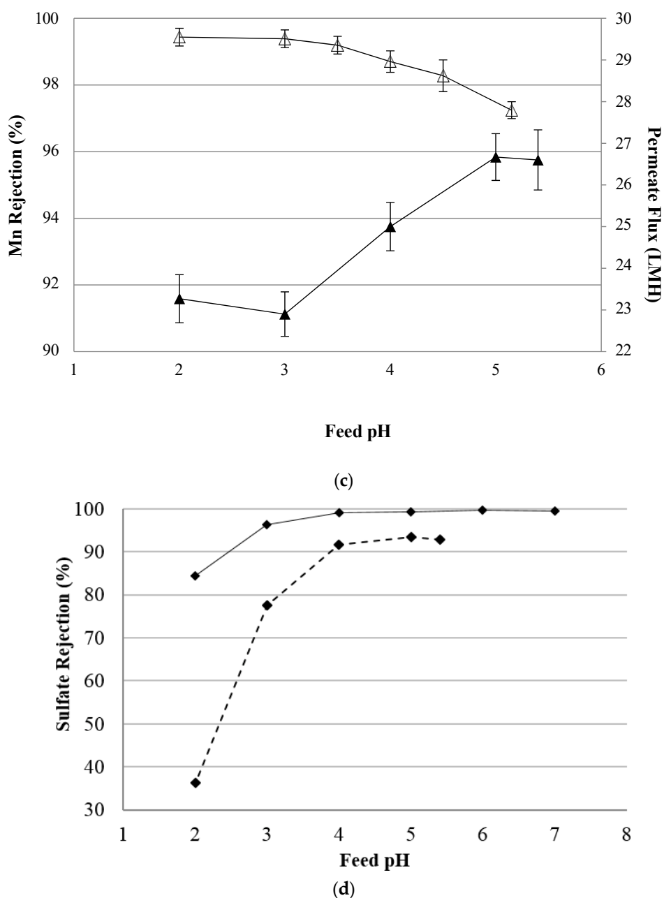
Figure 3. (a) Effect of feed pH on magnesium rejection (open symbol) and permeate flux (closed symbol). (Experimental conditions: \text{MgSO}_4 = 4000 mg/L, feed pressure = 10 bar, T = 25^\circ\text{C} ). (b) Effect of feed pH on copper rejection (open symbol) and permeate flux (closed symbol) (Experimental conditions: \text{CuSO}_4 = 100 mg/L, feed pressure = 10 bar, T = 25^\circ\text{C} ). (c) Effect of feed pH on apparent manganese rejection (open symbol) and permeate flux (closed symbol). (Experimental conditions: \text{Mn}(\text{NO}_3)_2 = 165 mg/L, feed pressure = 10 bar, T = 25^\circ\text{C} ). (d) Effect of feed pH on apparent sulfate rejection. Feed solution containing 4000 mg/L \text{MgSO}_4 (full line) and 100 mg/L \text{CuSO}_4 (dotted line). (Experimental conditions: feed pressure = 10 bar, T = 25^\circ\text{C} ).
