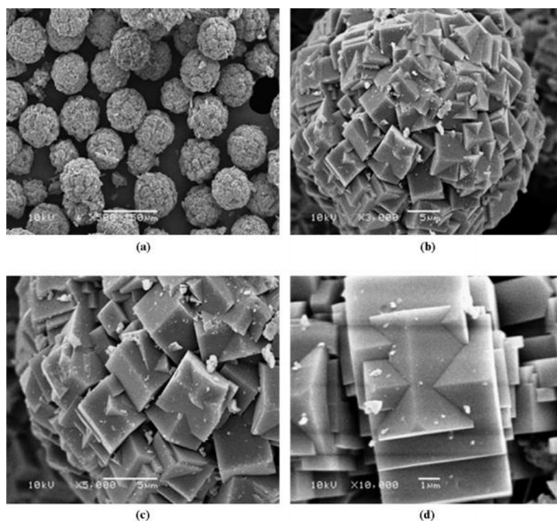
Figure 2. SEM micrographs of the ZSM-5 samples with an Si/Al ratio of 100 and different magnifications: (a) 500 \times , (b) 3K \times , (c) 5K \times , and (d) 10K \times (Reprinted from Applied Catalysis A: General, v. 374, issues 1-2, M. L. Mignoni, M. O. de Souza, S. B. C. Pergher, R. F. de Souza, K. Bernardo-Gusmão, Nickel oligomerization catalysts heterogenized on zeolites obtained using ionic liquids as templates, pp. 23–30, Copyright (2009), with permission from Elsevier B. V.) [55].
