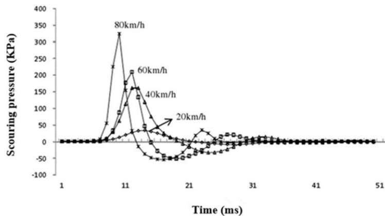
Figure 5. The variation of scouring pressure with time at different speeds.
